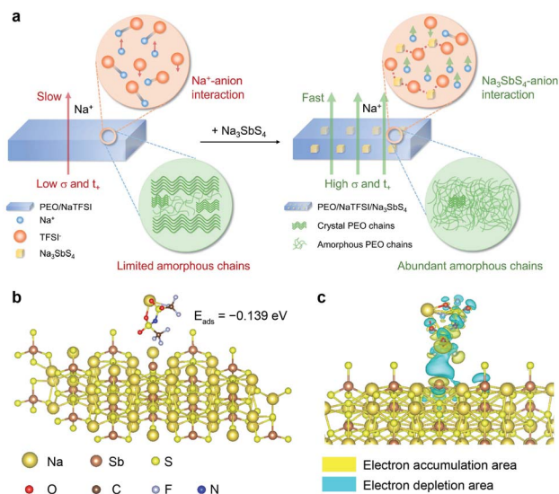
Fig. 1 Design of the interaction between the anion in salt and the additive. (a) Schematic illustrations of the PEO/NaTFSI and PEO/NaTFSI/ \text{Na}_3\text{SbS}_4 electrolytes where the interactions between \text{Na}_3\text{SbS}_4 and \text{TFSI}^- anions are highlighted by red dotted lines. (b) The optimized configuration, adsorption energy, and (c) differential charge density of NaTFSI adsorbed on \text{Na}_3\text{SbS}_4 ; the isosurface value is set to 0.0001 \text{ e Bohr}^{-3} .
