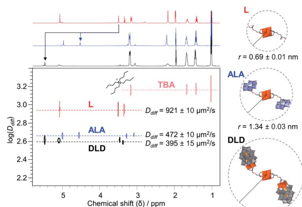
Fig. 6 Overlaid ^1\text{H} 2D DOSY NMR spectra of L, ALA and DLD labelled with the translational diffusion coefficient ( D_{\text{diff}} ) used to determine the hydrodynamic radius ( r ) for each structure, as shown on the right, and the corresponding ^1\text{H} 1D NMR spectra shown at the top.
