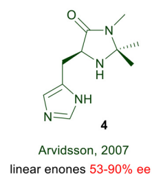
Scheme 4 Conjugate additions using pyrrolidines and imidazolidine catalysts.
