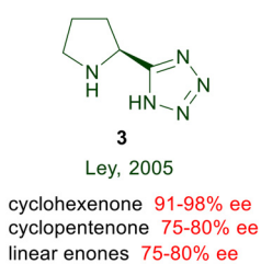
Scheme 4 Conjugate additions using pyrrolidines and imidazolidine catalysts.
