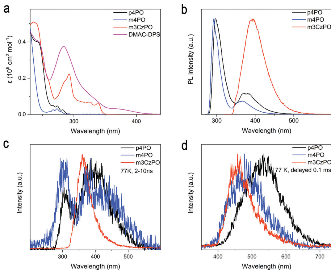
Fig. 4 (a) Absorption spectra recorded in dichloromethane ( 1.0 \times 10^{-6} \text{ M} ) at room temperature; (b) photoluminescence spectra recorded in transient PL decay of p4PO , m4PO and m3CzPO in dichloromethane ( 1.0 \times 10^{-6} \text{ M} ) at room temperature; (c) time-resolved fluorescence spectra (2–10 ns) in dilute 2-methyltetrahydrofuran ( 1.0 \times 10^{-6} \text{ M} ) at 77 K; and (d) time-resolved phosphorescence spectra (delayed 0.1 ms) in 2-methyltetrahydrofuran ( 1.0 \times 10^{-6} \text{ M} ) at 77 K.
