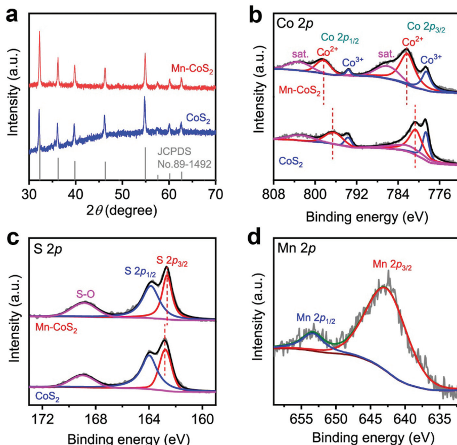
Fig. 3 Structural characterization of the as-prepared CoS 2 and Mn-CoS 2 : (a) XRD patterns; high-resolution XPS (b) Co 2p, (c) S 2p, and (d) Mn 2p spectra.
