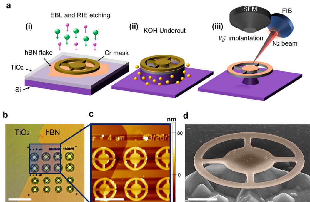
Fig. 1 Fabrication of hBN/ \text{TiO}_2 hybrid resonator. (a) Schematic representation of the fabrication process: (i) lithography step to pattern a Cr metal mask (brown steering-wheels) on hBN/ \text{TiO}_2 heterostructure and then transferring the mask into the heterostructure using ICP/RIE. Green and pink balls represent \text{SF}_6 , and Hydrogen species used in the latter step, respectively. (ii) Undercut of hBN/ \text{TiO}_2 hybrid resonator using 10% KOH aqueous solution. (iii) Generation of spin defects in hBN using angled Nitrogen focused ion beam (FIB). (b) Optical image of aligned EBL pattern on the hBN/ \text{TiO}_2 heterostructure. Scale bar: 25 \mu\text{m} . (c) AFM image of the patterned area. Scale bar: 10 \mu\text{m} . (d) 52° Tilted SEM image of the final hBN/ \text{TiO}_2 hybrid resonator. The false color shows the microring. Scale bar: 2 \mu\text{m} .
