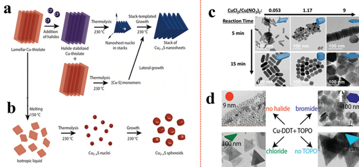
Fig. 1 (a) Schematic of controlling the 2D shape of the Cu 2-x S using Cl - source. The Cl - stabilized the lamellar Cu-alkanethiolate structure close to the nucleation stage influencing a 2D templated nucleation; (b) in the absence Cl - the lamellar structure melts and provides monomers for Cu 2-x S nuclei formation resulting in spheroids. Reproduced from ref. 49 with permission from ACS, copyright 2016; (c) effect of ratio variation between CuCl 2 and Cu(NO 3 ) 2 on morphology control of Cu 2-x S. Reproduced from ref. 90 with permission from ACS, copyright 2017; (d) effect of SnX 4 (X = Cl, Br) additives on nanoplate formation of Cu 2-x S. The Br - source formed hexagonal plates whereas the Cl - source produced triangular plates. Reproduced from ref. 91 with permission from ACS, copyright 2016.
