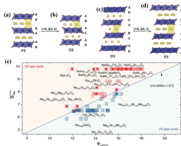
Fig. 2 Schematic diagram of the crystal structure of layered \text{Na}_x\text{TMO}_2 oxides for (a) P2 type, (b) O2 type, (c) O3 type and (d) P3 type. The blue and yellow spheres represent transition metals and \text{Na}^+ , respectively. Adapted with permission. 10 Copyright 2017, Wiley-VCH. (e) Cation potential of representative P2 and O3 sodium ion layered oxides. Adapted with permission. 33 Copyright 2020, American Association for the Advancement of Science.
