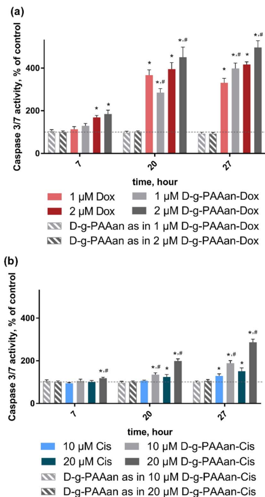
Fig. 6 Caspase 3/7 activity in LLC cells, incubated with: (a) either free Dox, free D-g-PAAAn or D-g-PAAAn-Dox at concentrations used in D-g-PAAAn-Dox nanoparticles (1 and 2 \mu M Dox); (b) either free Cis, free D-g-PAAAn or D-g-PAAAn-Cis at concentrations used in D-g-PAAAn-Cis nanoparticles (10 and 20 \mu M Cis); * p < 0.05 compared to control; # p < 0.05 compared to free drugs.
