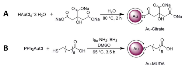
Scheme 2 Au NP synthesis via (A) the citrate reduction method according to Mattern et al. 17 yielding in 14 nm Au-citrate NPs and (B) a modified version of Stucky et al. 30 in order to obtain slightly smaller Au-MUDA NPs between 8–10 nm.
