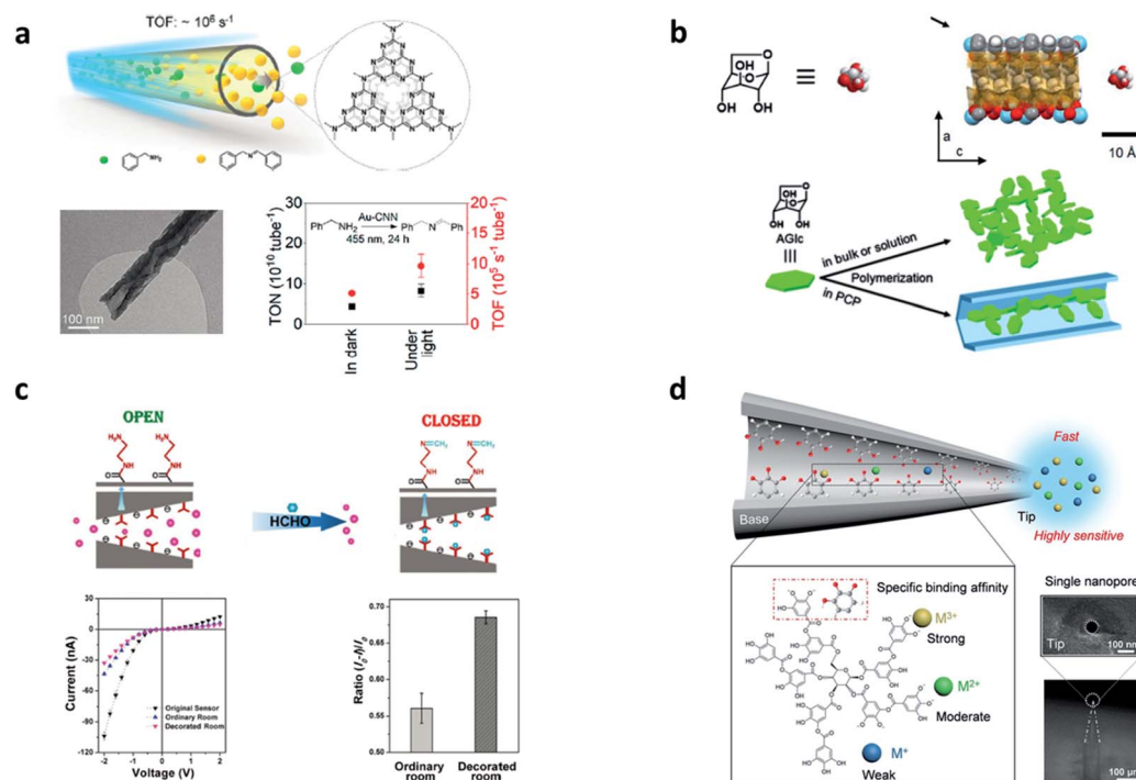
Fig. 5 Catalytic reaction systems in artificial nanochannels. (a) Schematic illustration of flow photocatalytic reactions in nanochannels. TEM image of a single Au carbon nitride nanotube. Turnover number (TON) and turnover frequency (TOF) of benzylamine oxidation under different reaction conditions. Reproduced with permission. 66 Copyright 2021, American Chemical Society. (b) Schematic illustration of the nanochannel structure and reactants. Polymerization of 6-anhydro- \beta -D-glucose (AGlc) in the bulk environment compared to nanochannels of porous coordination polymers (PCPs). Reproduced from ref. 32 with permission from the Royal Society of Chemistry. (c) The two states (open and closed) of the gating performance of the nanochannels. Current changes of the EDA-modified nanochannels with and without HCHO. The ionic current ratios of the EDA-modified and original nanochannels after interaction with HCHO in different current directions. Reproduced with permission. 83 Copyright 2019, Wiley. (d) Schematic illustration of a tannic acid-modified single nanochannel and binding energies with different ions. SEM images of the single conical nanochannel. Reproduced with permission. 21 Copyright 2020, Elsevier.
