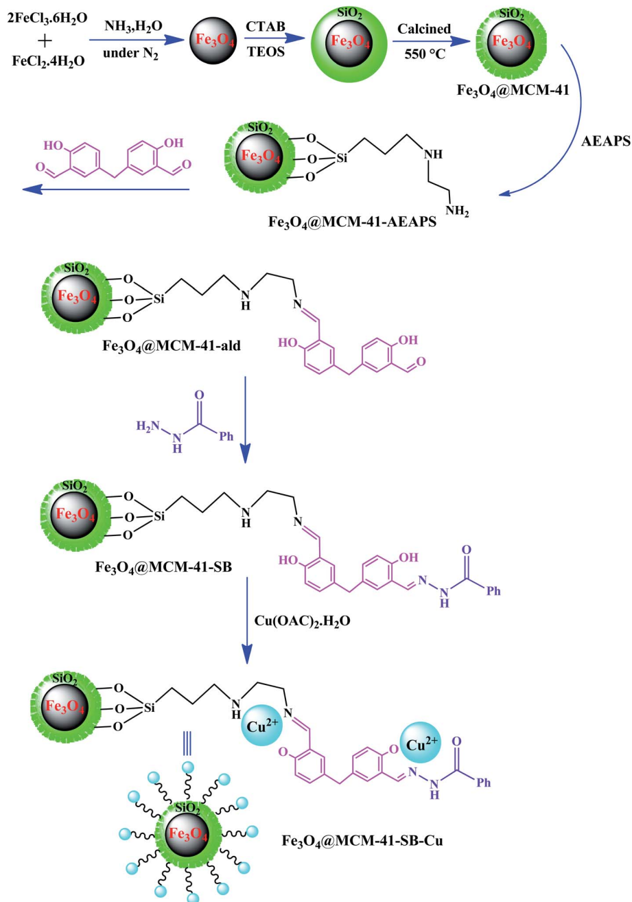
Fig. 12 Synthetic route of functionalized magnetic \text{Fe}_3\text{O}_4@MCM-41\text{-SB-Cu} hybrid catalyst. This figure was adapted with permission from Applied Organometallic Chemistry , 2020, 34 , e5572. 98
