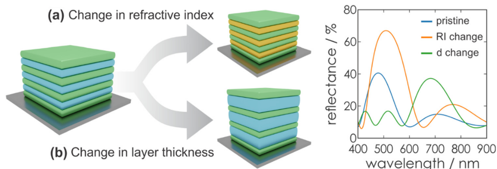
Fig. 6 Schematic illustration of the possible sensing mechanisms in a 1DPC. Upon exposure towards an analyte either the refractive index change (top) or the layer thickness change (bottom) is predominant. (a) Calculated red-shift of the Bragg peak (orange graph) induced by a change in the RI upon exposure towards a stimulus. The low RI was fixed to n_l = 1.6 while the high RI was changed from n_h = 1.8 to n_h = 2.0 . The thickness of each layer was 70 nm. (b) Calculated red-shift of the Bragg peak (green graph) induced by a change in the layer thickness upon exposure towards a stimulus. The low RI was fixed to n_l = 1.6 and the high RI was fixed to n_h = 1.8 while the layer thickness of the high RI material was changed from 70 to 140 nm. Note that the reflectance spectra in (a) and (b) were calculated for a glass substrate with n = 1.51 and a thickness of 1 mm.
