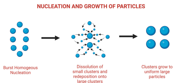
Fig. 2 Schematic illustration of nucleation and growth of nanoparticles leading to Ostwald ripening. Adapted from ref. 47.
