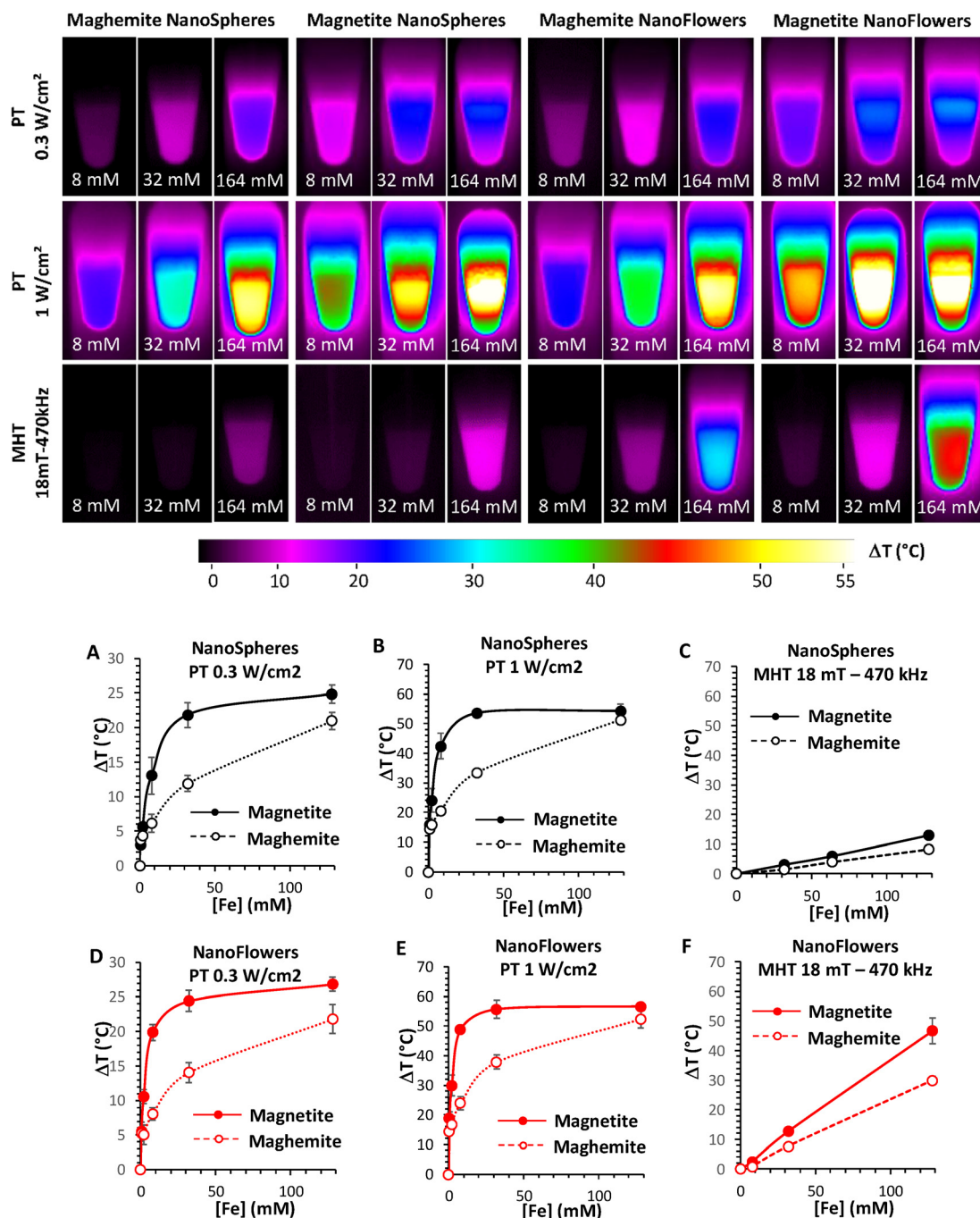
Fig. 13 (Upper images) Infrared images of 50 μL of magnetite and maghemite nanospheres and nanoflowers at different concentrations (8, 32 and 164 mM) for 10 min of exposure to different stimuli (Photothermal, or PT, at laser powers of 0.3 and 1 W cm -2 ; and magnetothermal, or MHT, at magnetic fields of 18 mT-470 kHz). (Lower images) Elevated-temperature profiles of magnetite and maghemite nanospheres (Panels A, B and C) and nanoflowers (Panels D, E and F) for PTT (Panels A, B, D and E) and MHT (Panels C and F). 104 Reprinted with permission under Creative Common Attribution 4.0 International License. Copyright 2020, Multidisciplinary Digital Publishing Institute.
