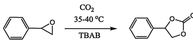
Scheme 11 The cycloaddition of \text{CO}_2 with styrene oxide using \text{Cu}_x\text{O}_y@COF . Reproduced with permission from ref. 26; copyright: 2019, Journal of CO 2 Utilization.
