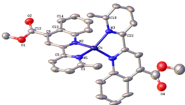
Fig. 6 Molecular structure of the cation of complex [\text{Cu}(6\text{'-Mepqcame})_2][\text{PF}_6]\cdot\text{CHCl}_3\cdot 0.13\text{H}_2\text{O} ( 6\text{'-CHCl}_3\cdot 0.13\text{H}_2\text{O} ); ellipsoids are plotted at the 30% probability level. H atoms, except those in the COOH groups, and the co-crystallized solvents are omitted for clarity.
