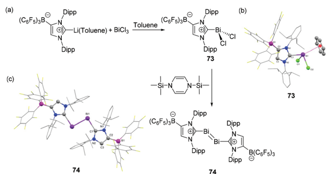
Fig. 24 (a) Syntheses of NHC-stabilized bismuth adduct 73 , and bis-muthene compound 74 ; solid-state structures of 73 (b) and 74 (c).
