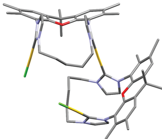
Fig. 4 X-ray crystal structure (sticks representation for improved clarity) of [[\text{Au}(\text{AuCl})_2(\text{Cl})]_2(\mathbf{16})] (colour code: Au yellow, Cl green, O red, N blue, H not displayed). Important bond lengths (pm) and angles (°): Au...Au 586.2(1), 572.8(1), 660.6(1), Au–C(NHC) 197(2), 198(2), 199(2), Au–Cl 28.4(4), 226.1(5); Cl–Au–C(NHC) 177.2(6), 178.2(6), C(NHC)–Au–C(NHC) 177.3(7).
