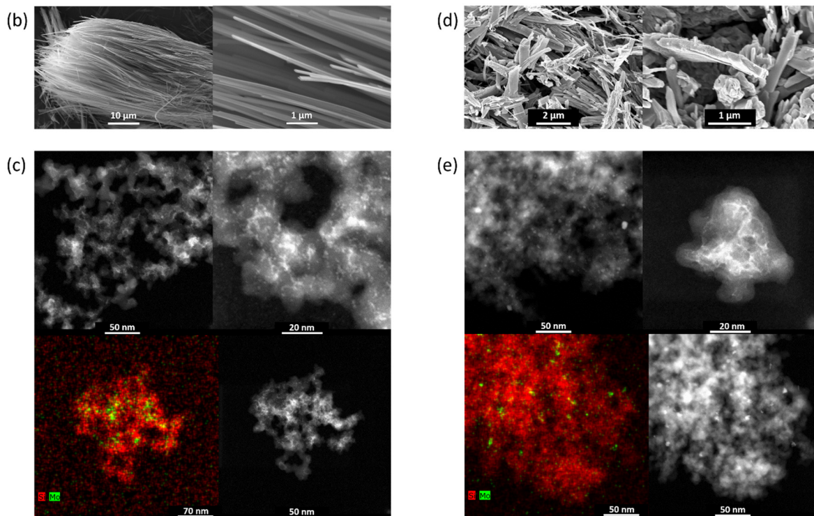
Fig. 1 a) Synthesis of Mo 2 C-nb from \alpha -MoO 3 -nb and Mo 2 C/SiO 2 from silica-supported delaminated MoO 3 films MoO 3 /SiO 2 ; b) SEM images of as synthesized \alpha -MoO 3 -nb; c) HAADF-STEM images and EDX elemental (Si and Mo) maps of MoO 3 /SiO 2 ; d) SEM images of Mo 2 C-nb; and e) HAADF-STEM images and EDX maps of Mo 2 C/SiO 2 .
