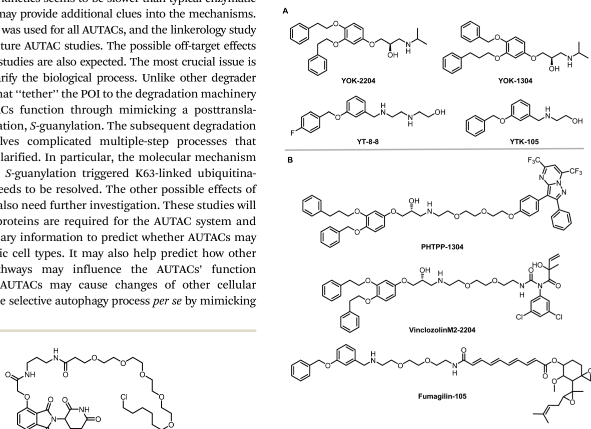
Fig. 19 AUTOTAC compounds. (A) p62zz-binding compounds used as AUTOTAC's warheads; (B) AUTOTACs including PHTPP-1304 targeting ER \beta , vinclozolinM2-2204 targeting AR and fumagilin-105 targeting MetAP2.
