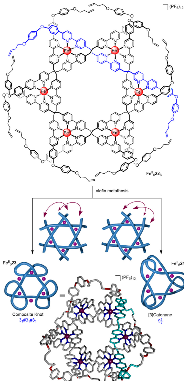
Fig. 8 A hexameric circular helicate and its closure to give molecular composite knot \text{Fe}_6^{\text{II}} \mathbf{23} and link \text{Fe}_6^{\text{II}} \mathbf{24} . 58
