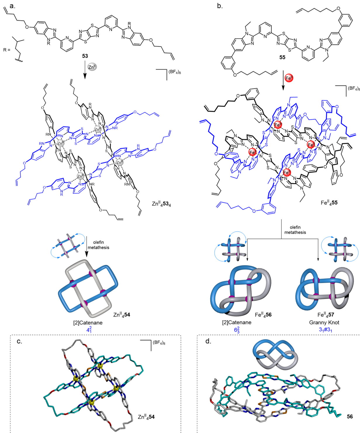
Fig. 20 Synthesis of 2 \times 2 interwoven molecular grids and their closures by olefin metathesis to generate (a) Solomon link 54 , 14 or (b) 6^3_3 link 56 and granny knot 57 , 15 X-ray crystal structures of (c) \text{Zn}^{\text{II}}_4\mathbf{54} and (d) demetallated link 56 .
