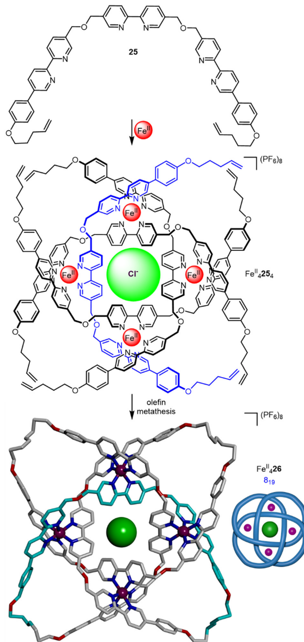
Fig. 9 Synthesis of 8_{19} knot \text{Fe}_4^{\text{II}} \mathbf{26} via braiding of three ligand strands. 59
