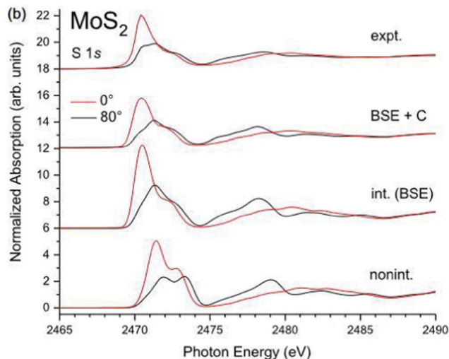
Fig. 11 K-Edge XAS of \text{MoS}_2 calculated within the non-interacting approximation (bottom), BSE (second curves), and BSE + cumulant (third curves), compared to experiment (top). The angle of polarization is shown by the colors. Reprinted figure with permission from [J. C. Woicik, C. Weiland, A. K. Rumaiz, M. T. Brumbach, J. M. Ablett, E. L. Shirley, J. J. Kas and J. J. Rehr, Phys. Rev. B , 2020, 101 , 245105], Copyright (2022) by the American Physical Society.
