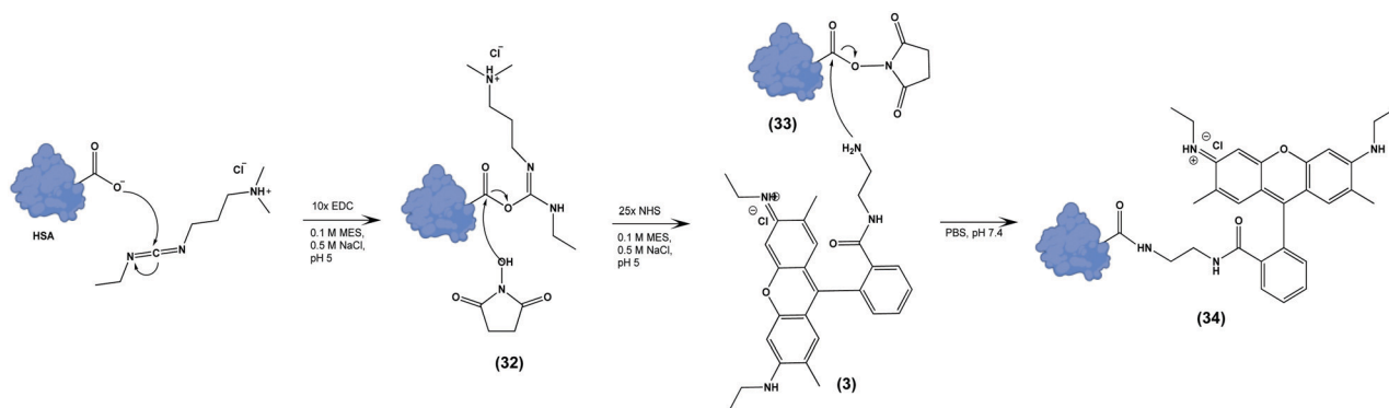
Scheme 3 Terminal carboxylate residues of human serum albumin (HSA) are functionalized with (3) by EDC/NHS yielding pH-sensitive fluorescent HSA (34).
