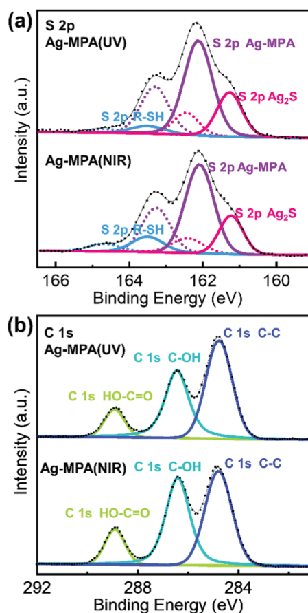
Fig. 3 High-resolution XP-spectra of Ag-MPA (UV) and Ag-MPA (NIR) (a) S\ 2p , solid lines represent the signals stemming from S\ 2p_{3/2} , dash lines represent the signals stemming from S\ 2p_{1/2} ; (b) C 1s.
