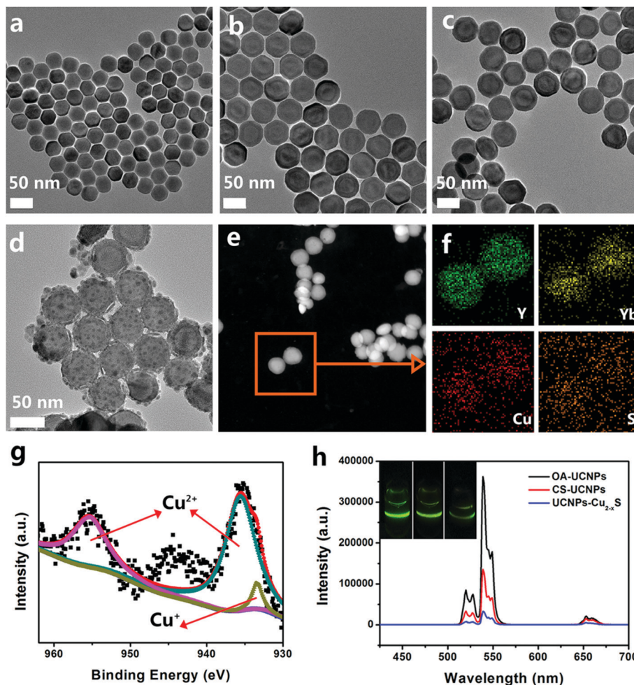
Fig. 1 TEM images of (a) NaYF 4 :Yb/Er, (b) NaYF 4 :Yb/Er@NaYF 4 :Yb UCNPs, (c) CS-UCNPs, and (d) UCNP-Cu 2-x S. (e) HAADF-STEM image of UCNP-Cu 2-x S and (f) the corresponding element mappings. (g) XPS of Cu in UCNP-Cu 2-x S. (h) UCL spectra of OA-UCNPs, CS-UCNPs, and UCNP-Cu 2-x S excited by a 980 nm NIR laser. Insets are the corresponding digital photographs of the solutions irradiated by the 980 nm NIR laser.
