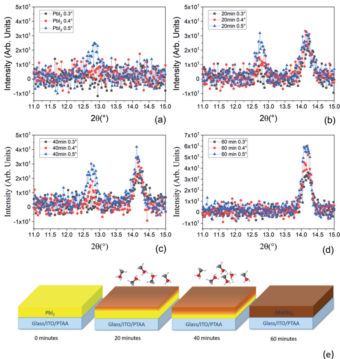
Fig. 5 (a) XRD patterns collected in grazing incidence configuration at three different incidence angles, namely 0.3°, 0.4° and 0.5° for the PbI 2 deposited sample, (b) after 20 minutes, (c) 40 minutes and (d) 60 minutes of MAI deposition on ITO/PTAA substrates. (e) Schematic representation of the conversion mechanism from PbI 2 to MAPbI 3 during the MAI deposition step. In the pristine sample only the PbI 2 peak is detected at 2\theta = 12.67^\circ . Along the MAI deposition step, the conversion of PbI 2 to MAPbI 3 starts from the topmost part of the film toward the bottom until the complete conversion has occurred.
