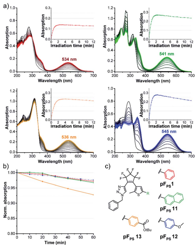
Fig. 5 Photochromic properties of various thienyl substitutions: (a) time-dependent changes of the absorption spectra of 60 \mu\text{M} solutions of pFps 1, 11–13 upon UV light irradiation (310 nm, LED) in chloroform towards the (pseudo)-photostationary state; insets show the absorption vs. time trace measured at the VIS absorption maximum during extended UV irradiation to analyse the photostability, (b) thermostability (20 ^{\circ}\text{C} ) of the CF isomers, (c) structures.
