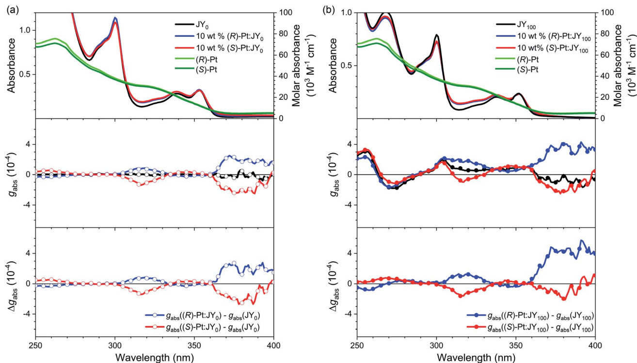
Fig. 4 (a) UV-vis absorption (top), g_{abs} (middle), and the g_{abs} difference spectra (bottom; \Delta g_{abs} , g_{abs}(10 \text{ wt}\% \text{ Pt}:JY_0) - g_{abs}(JY_0) ) for the JY_0 films (quartz substrates) in the absence and presence of 10 wt% (R)-Pt or 10 wt% (S)-Pt. (b) UV-vis absorption (top), g_{abs} (middle), and the g_{abs} difference spectra (bottom; \Delta g_{abs} , g_{abs}(10 \text{ wt}\% \text{ Pt}:JY_{100}) - g_{abs}(JY_{100}) ) for the JY_{100} films (quartz substrates) in the absence and presence of 10 wt% (R)-Pt or 10 wt% (S)-Pt.
