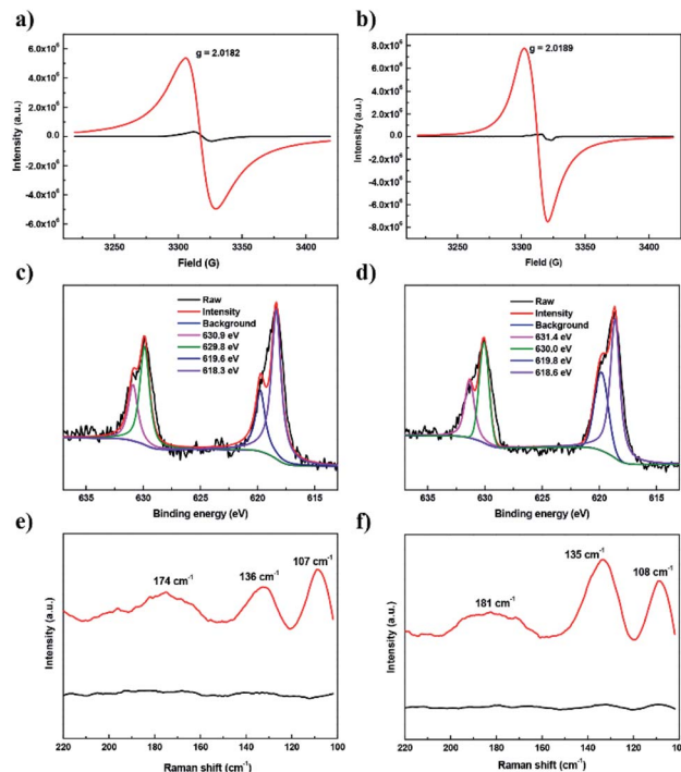
Fig. 5 Spectroscopy study. (a and b) EPR spectra of JUC-560 (a) and JUC-561 (b) before (black curve) and after (red curve) iodine uptake. (c and d) XPS of iodine for JUC-560 (c) and JUC-561 (d) after iodine uptake. (e and f) Raman spectra of JUC-560 (e) and JUC-561 (f) before (black curve) and after (red curve) iodine uptake.
