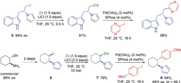
Scheme 2 Zn-Insertion to alkyl iodides bearing an indolyl NH-group and (or) a \beta -N-pyrrolyl group.
