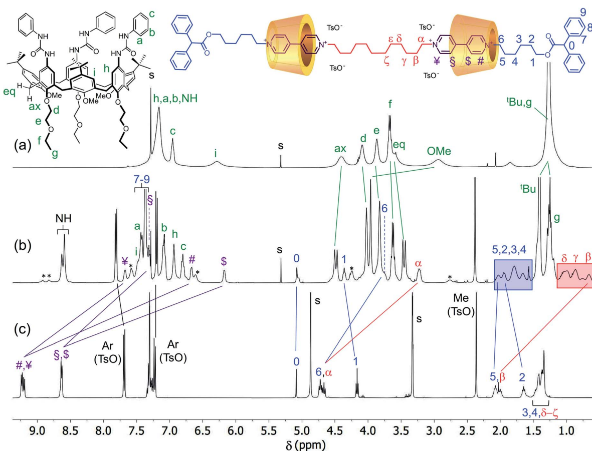
Fig. 3 1 H NMR stack plot (400 MHz, CDCl 3 ) of (a) wheel CX, (b) [3]rotaxane R6 UL , and (c) dumbbell 7a. For solubility reasons, spectrum (c) was taken in CD 3 OD. The most representative resonances are labelled according to the molecular sketches placed above the stack plot, while their complexation induced shifts are indicated with solid lines; the unlabeled signals marked with an asterisk in the spectrum (b) belong to a rotamer of R6 UL in the partial cone ( paCo ) conformation; see text and ESI † for further details.
