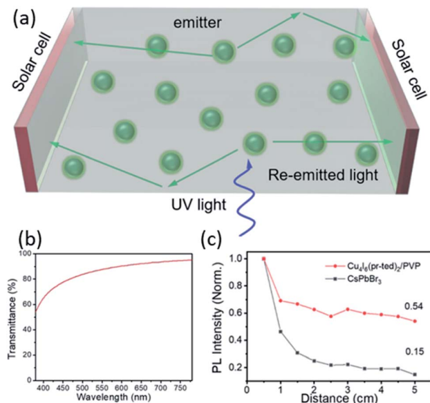
Fig. 7 (a) Schematic showing an LSC device using \text{Cu}_4\text{I}_6(\text{pr-ted})_2/\text{PVP} ink. Green balls: \text{Cu}_4\text{I}_6(\text{pr-ted})_2/\text{PVP} nanoparticles. (b) Light transmittance of prepared thin film in visible light region. (c) Comparison of PL intensities as a function of propagation lengths in the \text{Cu}_4\text{I}_6(\text{pr-ted})_2/\text{PVP} film and \text{CsPbBr}_3 nanocrystal film. Reproduced with permission from ref. 36. Copyright 2020, American Chemical Society.
