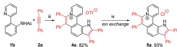
Scheme 2 Rh-Catalyzed cyclization of 2-(pyridin-2-yl)aniline ( 1 ) with 1,2-diphenylacetylene ( 2a ). Reaction conditions: (i) 1a (0.1 mmol), 2a (0.2 mmol), [\text{Cp}^*\text{RhCl}_2]_2 (5 mol%), and AgOTf (0.12 mmol) in t -AmOH (1.5 mL) at 120 °C for 24 h under \text{O}_2 ; (ii) 1a (0.1 mmol), 2a (0.2 mmol), [\text{Cp}^*\text{RhCl}_2]_2 (5 mol%), AgOTf (0.12 mmol), and \text{Ac}_2\text{O} (0.5 mmol) in t -AmOH (1.5 mL) at 120 °C for 24 h under \text{O}_2 ; (iii) 1b (0.1 mmol), 2a (0.3 mmol), [\text{Cp}^*\text{RhCl}_2]_2 (5 mol%), AgSbF 6 (20 mol%), \text{Cu}(\text{OAc})_2 \cdot \text{H}_2\text{O} (0.3 mmol) and TfOH (0.15 mmol) in t -AmOH (1.5 mL) at 140 °C for 24 h under \text{N}_2 ; (iv) column chromatography on ion exchange resin. t -AmOH = 2-methylbutan-2-ol. AgOTf = silver trifluoromethanesulfonate. TfOH = trifluoromethanesulfonic acid.
