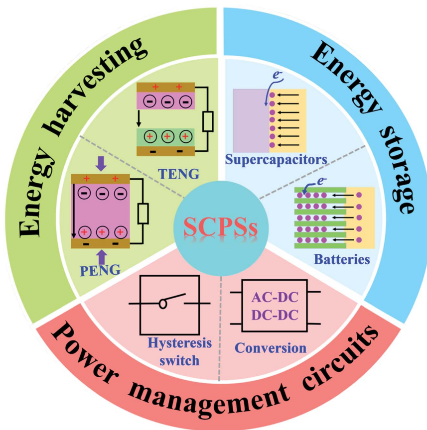
Fig. 1 Nanogenerator-based self-charging power systems (SCPSS) with three components: energy harvesting, energy storage and power management circuit.
