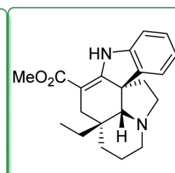
136 : (+)-Vincadifformine
