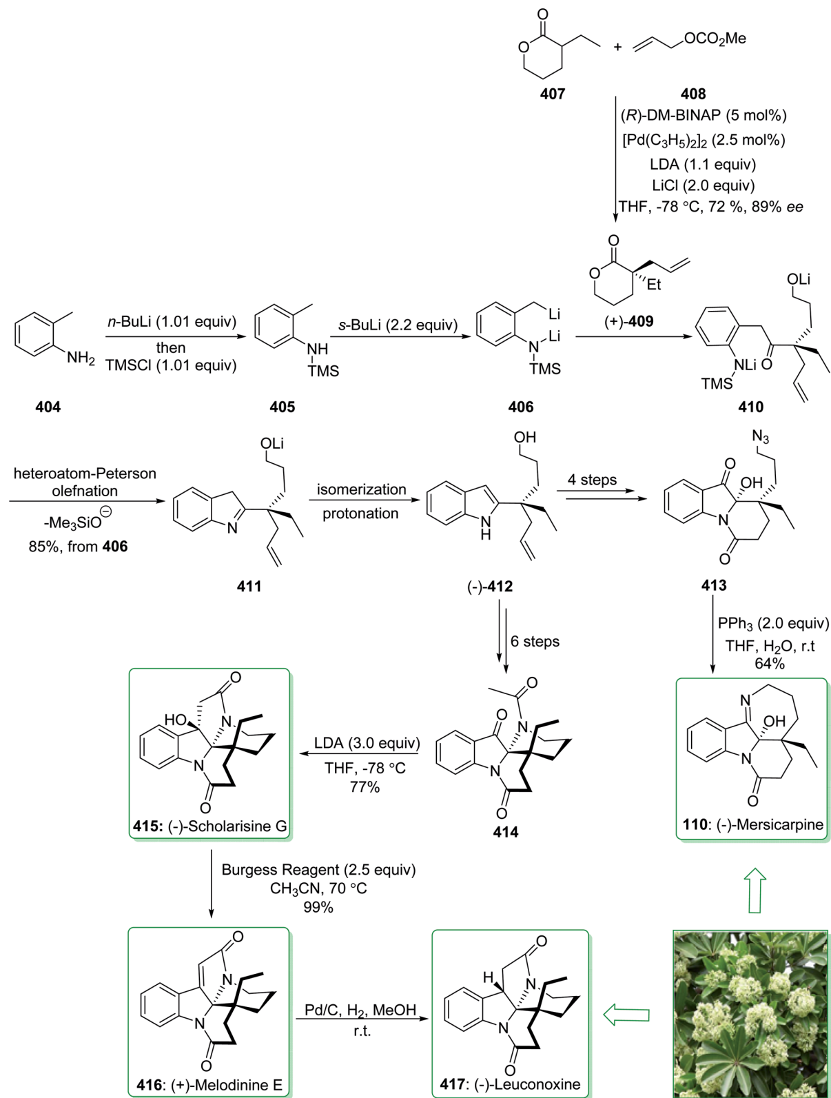
Scheme 57 Total synthesis of (–)-scholarisine G ( 415 ), (+)-melodinine E ( 416 ), (–)-leuconoxine ( 417 ) and (–)-mersicarpine ( 110 ).
