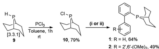
Scheme 1 The synthesis of ligands 1 and 2 , through reaction of phosphine chloride 10 with (i) 2-biphenylmagnesium bromide, CuCl 5 mol%, LiBr 10 mol%, toluene, 110 °C, 12 h and Ar; or (ii) (2',6'-dimethoxy-[1,1'-biphenyl]-2-yl)lithium, THF, -80 °C → RT, 24 h and Ar, respectively.
