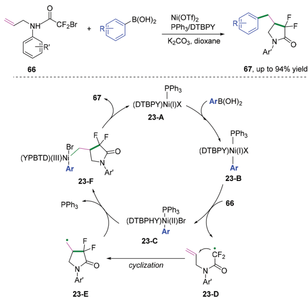
Scheme 36 Nickel-catalyzed \text{C}(\text{sp}^2)\text{-C}(\text{sp}^3) bond coupling cyclization.
