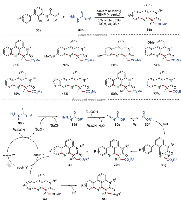
Scheme 30 The construction of ester-functionalized phenanthridines.
