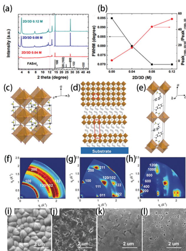
Fig. 5 (a) XRD patterns of THP films with different amount of PEA + incorporated. (b) FWHM of the (100) peaks of films with different amounts of 2D perovskites, and ratios of the (100) peak intensities of 2D/3D films to those of pristine 3D perovskites with different amounts of 2D perovskites incorporated. Schematic illustration of the crystal structures of (c) a 3D perovskite, (d) a 2D/3D perovskite and (e) a 2D PEA 2 SnI 4 perovskite. (f) GIWAXS images of samples at 65 °C recorded at an incident angle of 0.25° for (f) a 3D perovskite, (g) a 2D/3D mixed perovskite and (h) a 2D perovskite. (i–l) SEM images of FASnI 3 perovskites with different amount of the 2D Sn perovskite (0, 0.08, 0.012, and 0.16 M). 41 Copyright 2017, WILEY-VCH Verlag GmbH & Co. KGaA, Weinheim.
