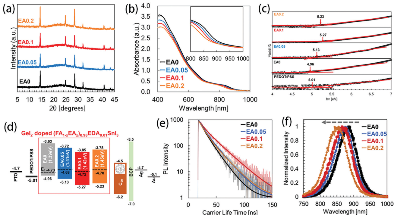
Fig. 6 (a) XRD patterns of \text{Gel}_2 doped (\text{FA}_{1-x}\text{EA}_x)_{0.98}\text{EDA}_{0.01}\text{SnI}_3 perovskite films with different amount of EA incorporated. (b) UV-Vis measurement of \text{Gel}_2 doped (\text{FA}_{1-x}\text{EA}_x)_{0.98}\text{EDA}_{0.01}\text{SnI}_3 perovskite films with different amount of EA incorporated. (c) The PYS measurement of perovskite films with different EA amount. (d) The schematic illumination of band alignment for the PSC with various EA amount. (e) Normalized PL spectra and (f) TRPL spectra of perovskite films with various EA amount. 14 Copyright 2020, Elsevier.
