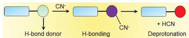
Fig. 8 Mode of interaction of hydrogen bonding motif-based gelators with cyanide.
