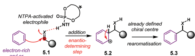
Scheme 52 General picture of an enantioselective Friedel–Crafts reaction. In this section, we considered those reactions in which the addition step is enantiodetermining.
