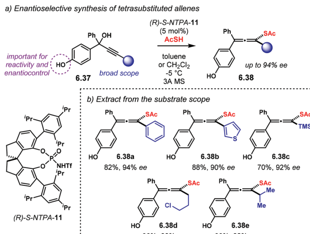
Scheme 74 (a) Enantioselective synthesis of tetrasubstituted allenes via an oQM, reported by the group of Sun. (b) Extract from the substrate scope. The reaction tolerates a wide variety of substituents.
