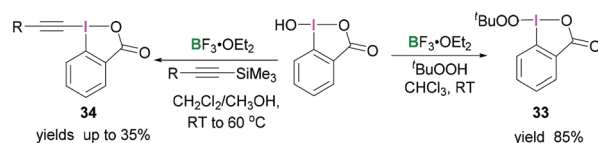
Scheme 13 Transformation of benziodaoxolone into the corresponding alkylperoxyiodinane 33 and alkynyl derivative 34.
