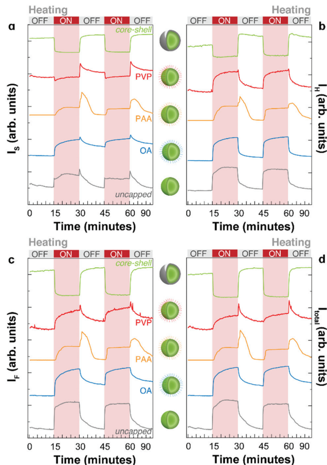
Fig. 3 The integrated intensity in two thermal cycles corresponding to the (a) S transition ( I_S , {}^4\text{S}_{3/2} \rightarrow {}^4\text{I}_{15/2} ), (b) H transition ( I_H , {}^2\text{H}_{11/2} \rightarrow {}^4\text{I}_{15/2} ), (c) F transition ( I_F , {}^4\text{F}_{9/2} \rightarrow {}^4\text{I}_{15/2} ), and (d) the sum of the areas of S, H, and F transitions ( I_{\text{total}} ) for all the samples studied in this work.
