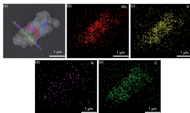
Fig. 3 (a) SEM and (b–e) elemental mapping images of \text{MoS}_2\text{@C@PANI} . Line-scan profiles are inserted in (a).
