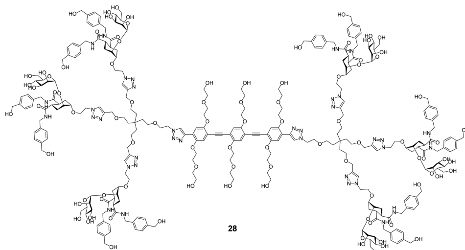
Fig. 11 Structure of hexavalent molecular rod Polyman26 (28).
