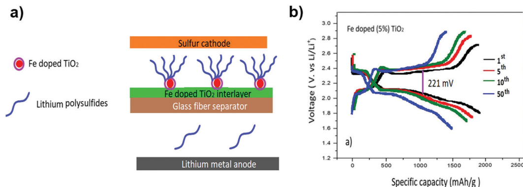
Fig. 28 (a) Schematic for the Li-S battery configuration with the Fe-doped \text{TiO}_2 interlayer on a glass fiber separator. (b) Discharge-charge voltage profiles of the Li-S cell with a 5% Fe-doped \text{TiO}_2 separator at 1 C. Image reprinted with the permission from ref. 144. Copyright © 2020, Elsevier License 5041340812636.
