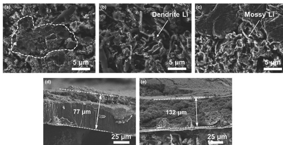
Fig. 5 SEM images of cycled Li anodes in Li|SPAN full cells after 50 cycles at 0.5\ \text{C} with (a) mixed-DIPE, (b) EC/DEC and (c) DOL/DME electrolytes. The corresponding cross-sectional SEM images of the Li foils with (d) mixed-DIPE and (e) EC/DEC. Image reprinted with the permission from ref. 68. Copyright © 2020, John Wiley and Sons License 5064250079974.
