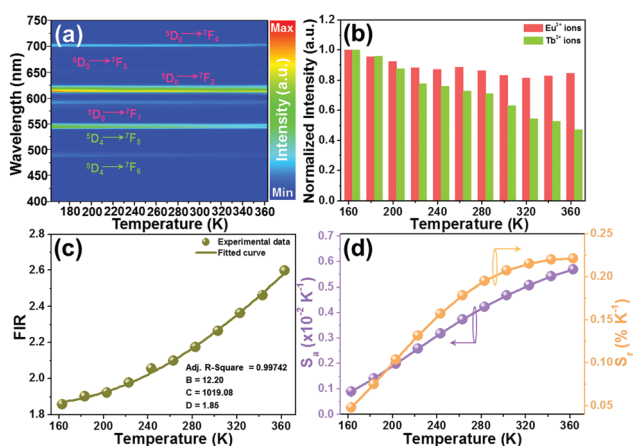
Fig. 5 (a) Thermal evolution emission spectra of \text{YMO}:\text{Tb}^{3+}/0.06\text{Eu}^{3+} NTE microparticles excited at 297 nm. (b) Normalized emission intensities of the \text{Eu}^{3+} and \text{Tb}^{3+} ions as a function of temperature. (c) Dependence of FIR value on temperature. (d) Temperature-dependent S_a and S_r values.
