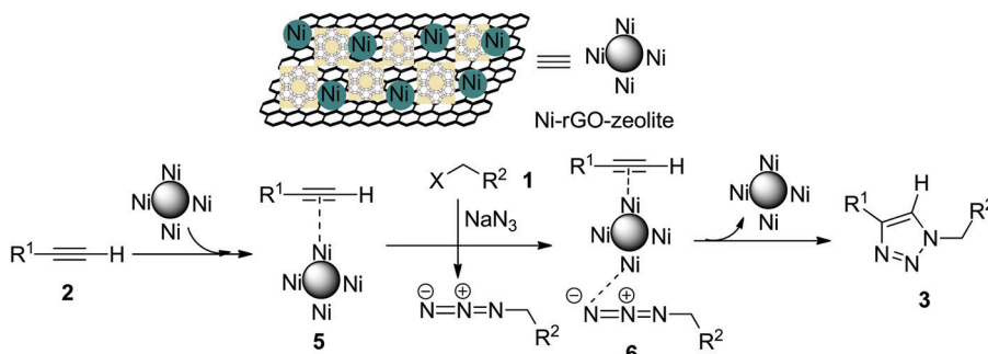
Scheme 2 Plausible mechanism for the Ni-rGO-zeolite catalysed click reaction (NiAAC).
