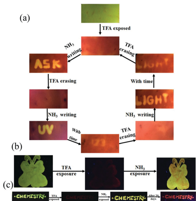
Fig. 10 Fabricating rewritable/self-erasable fluorescent platforms using 6-PMMA on (a) a filter paper, (b) a symbol on glass plate and (c) word writing on a glass plate ( \lambda_{\text{exc}} = 365 \text{ nm} ).
