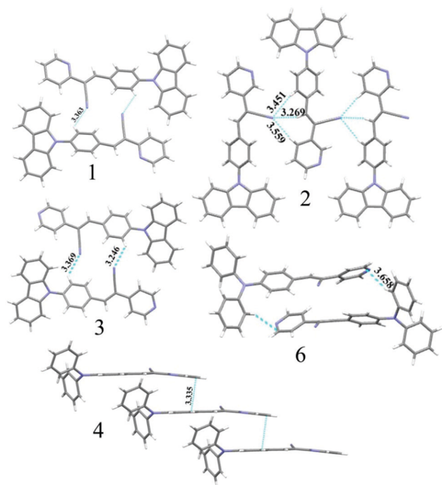
Fig. 7 Molecular interactions in the crystal lattice of 1–4 and 6. C (grey), N (blue) and H (white). Dotted lines indicate the hydrogen bonding, C–H \cdots N and \pi \cdots \pi interactions in Å.
